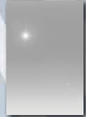
Silver Frost
